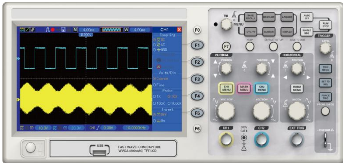
Front Panel of DSO-1000D
