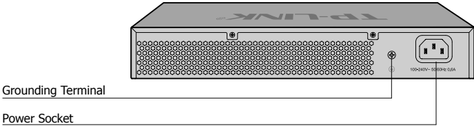
Figure 1-10 Rear Panel of TL-SG1024D/TL-SG1016D
