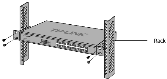
Figure 2-3 Rack Installation
