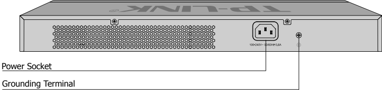
Figure 1-9 Rear Panel of TL-SG1024/TL-SG1016
