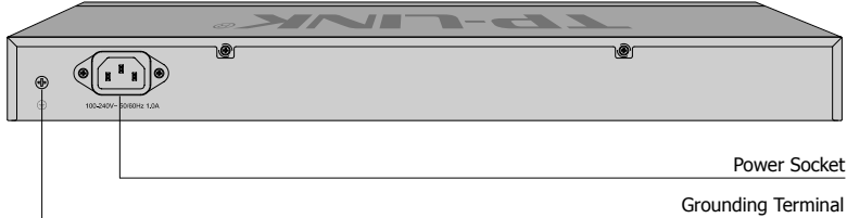
Figure 1-8 Rear Panel of TL-SG1048
