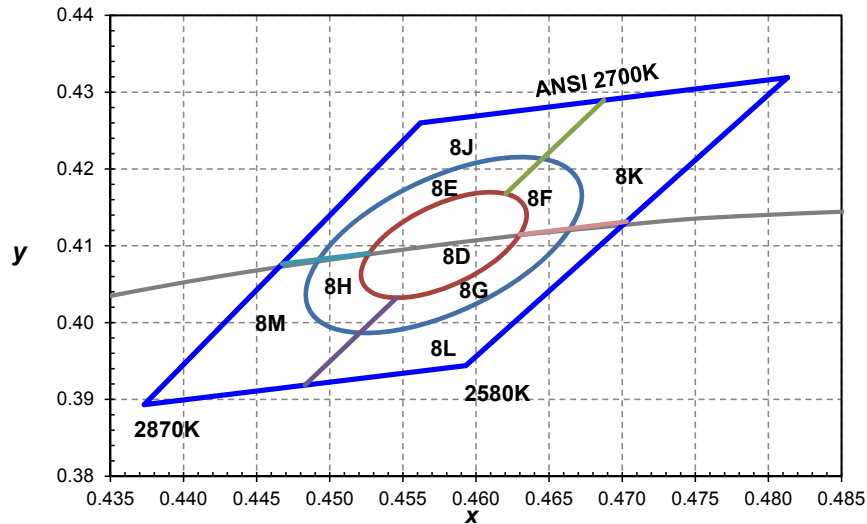
Figure 13. 2700K 1/9 th color bin structure.
