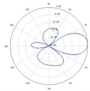
Horizontal Elevation
