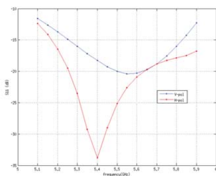
Return Loss
