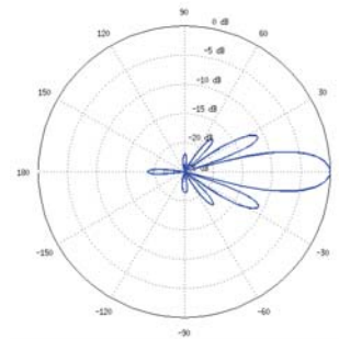
Horizontal Elevation
