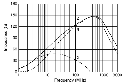
BLM21RK121SN1
