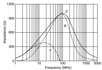
BLM21RK102SN1
