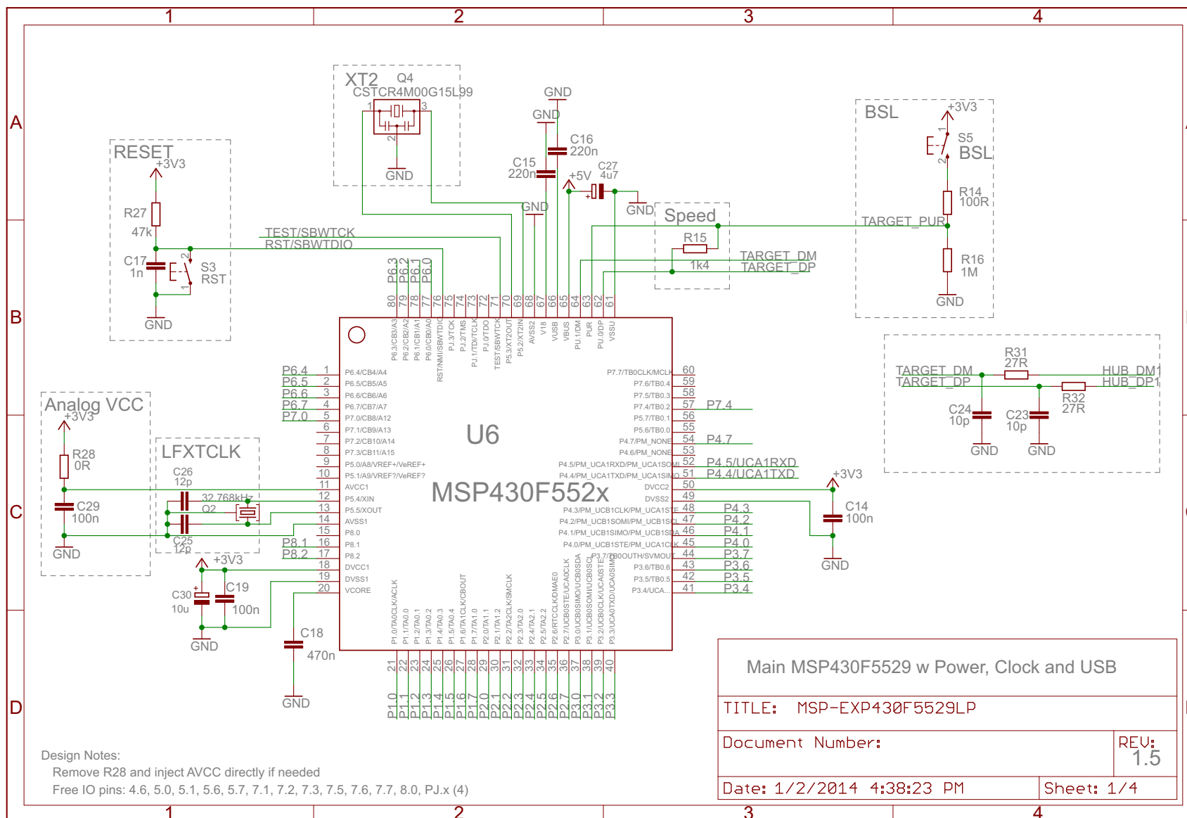
Figure 40. Schematics (1 of 4)
