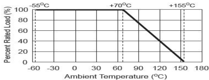
Derating Curve
