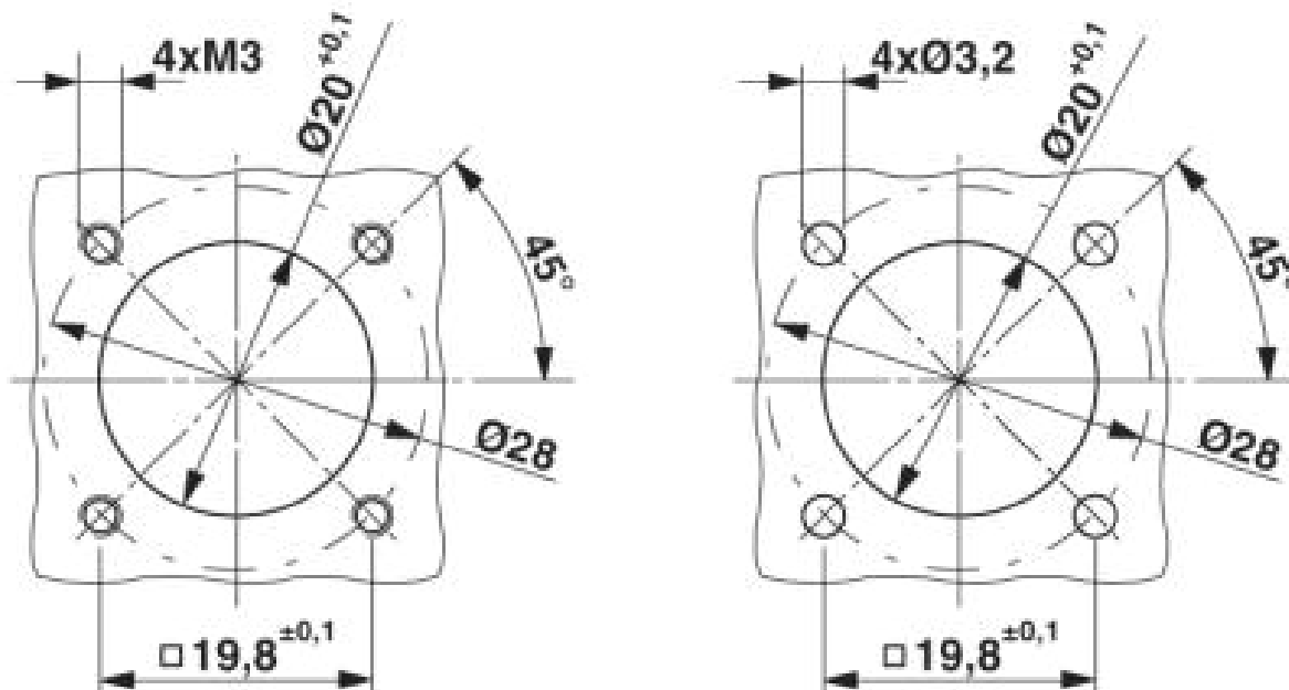
Installation dimensions
