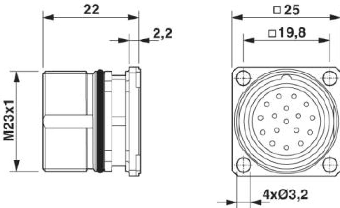
Dimensioned drawing
