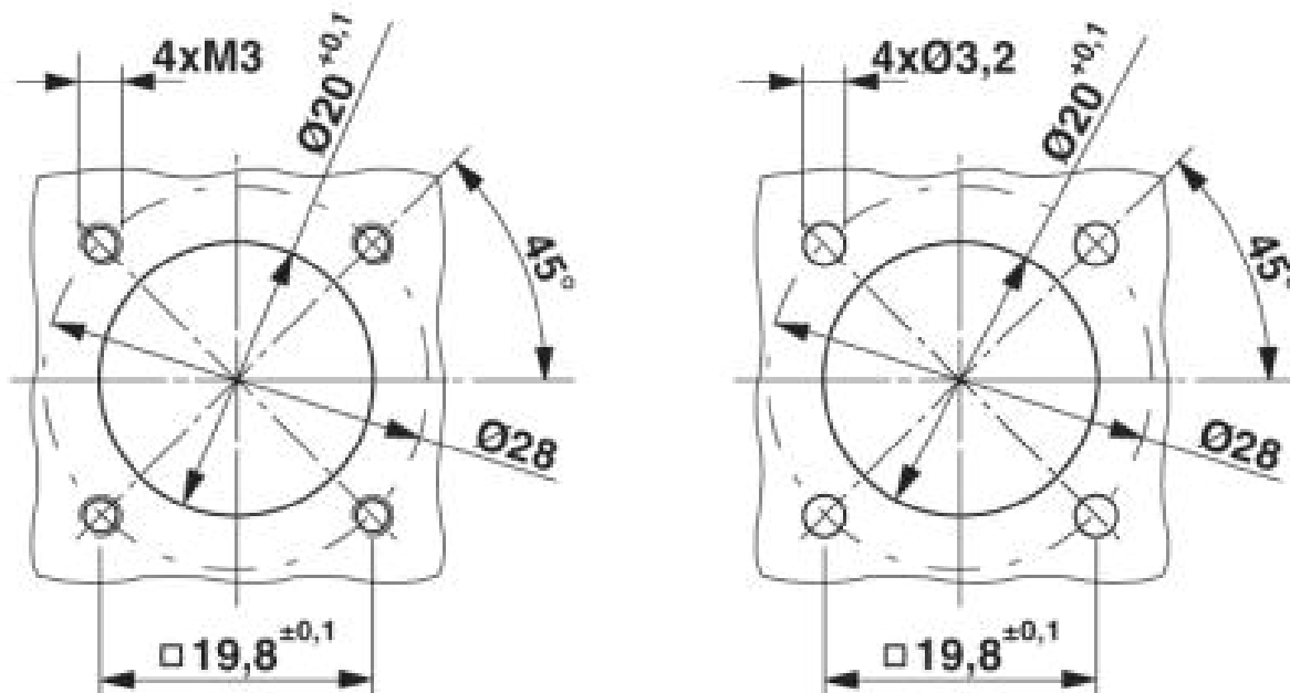
Installation dimensions
