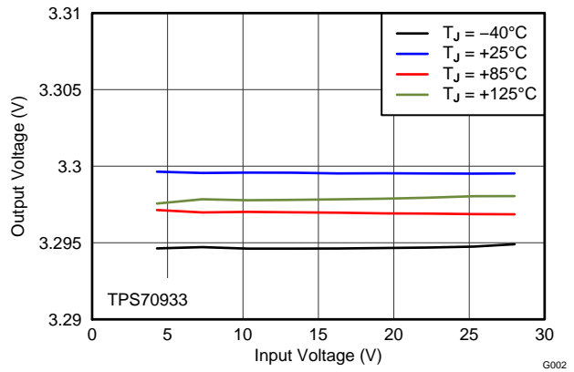
Figure 2. 3.3-V LINE REGULATION vs V_{IN} AND TEMPERATURE
