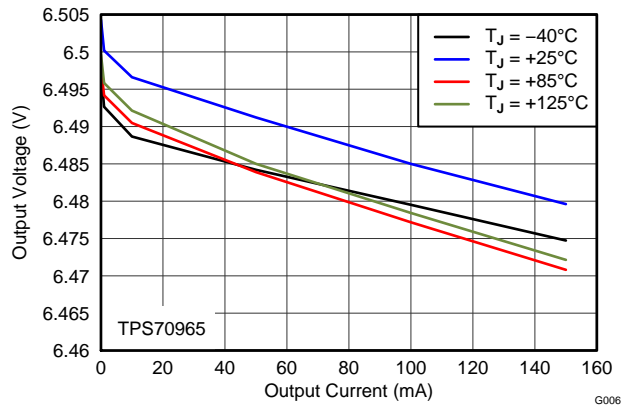
Figure 6. 6.5-V LOAD REGULATION vs I_{OUT} AND TEMPERATURE
