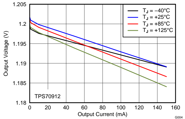
Figure 4. 1.2-V LOAD REGULATION vs I_{OUT} AND TEMPERATURE
