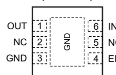
DRV PACKAGE 2-mm × 2-mm SON-6 (TOP VIEW)
