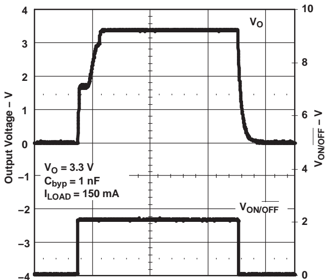
TURN-ON TIME
