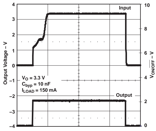
TURN-ON TIME
