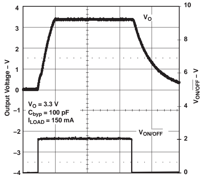
TURN-ON TIME
