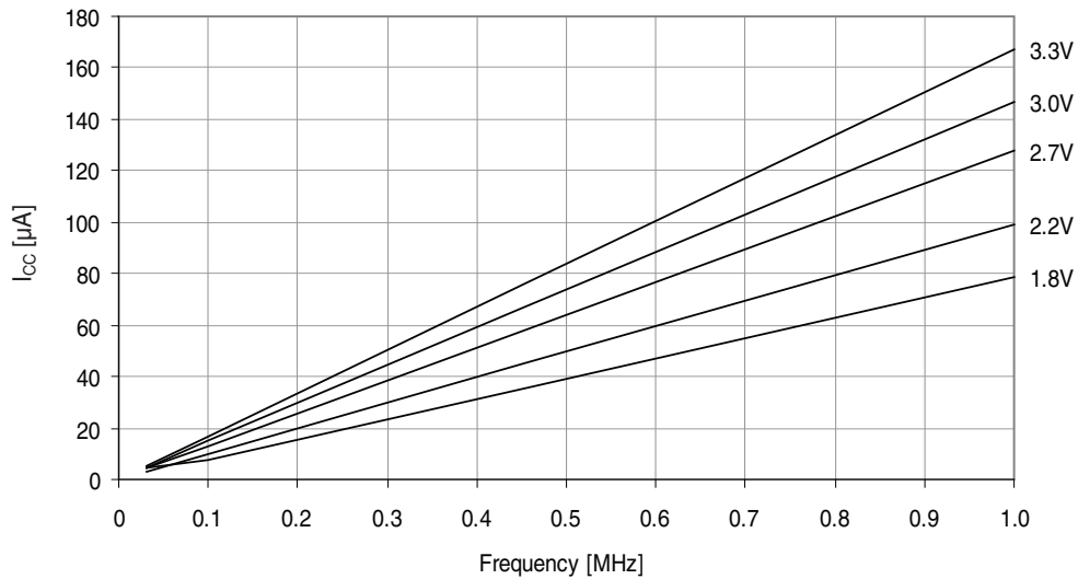
Figure 37-174. Idle mode supply current vs. frequency.
