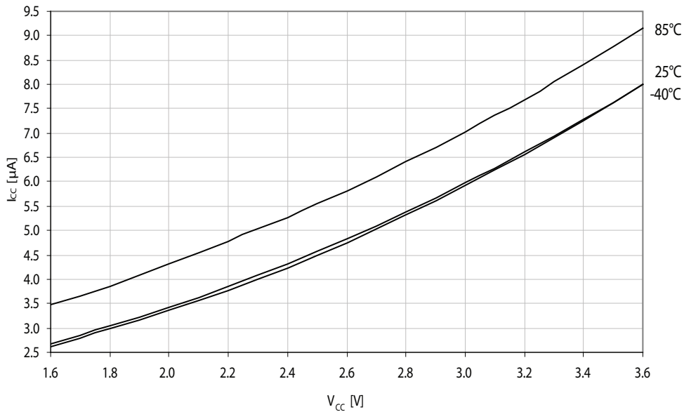
Figure 37-267. Standby supply current vs. V_{CC} . Standby, f_{SYS} = 1MHz .
