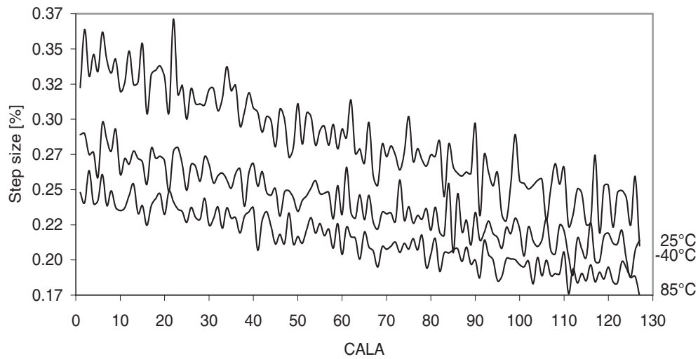
Figure 37-239. 2MHz internal oscillator CALA calibration step size.
