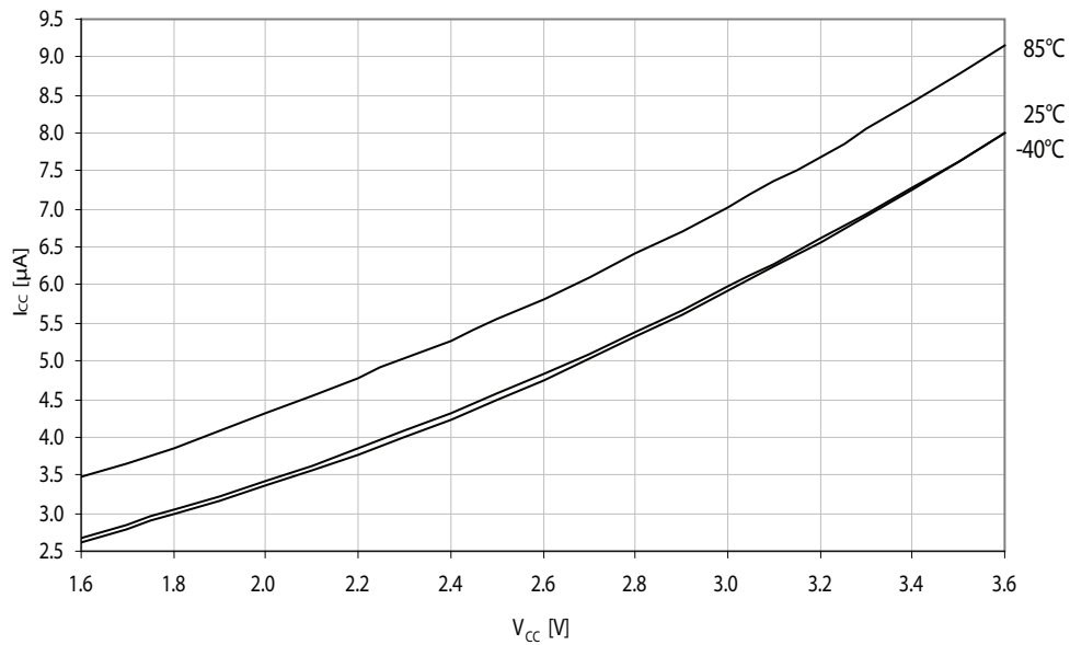
Figure 37-18. Standby supply current vs. V_{CC} . Standby, f_{SYS} = 1MHz .
