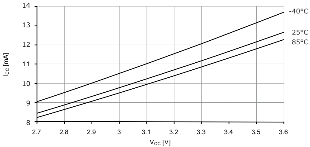
Figure 37-14. Idle mode current vs. V_{CC} .
