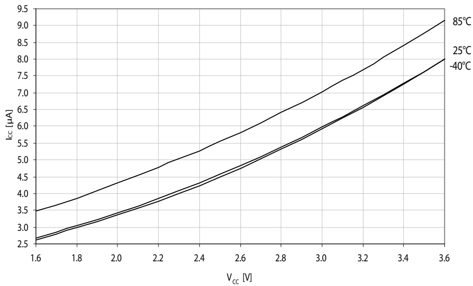
Figure 37-184. Standby supply current vs. V_{CC} . Standby, f_{SYS} = 1MHz .
