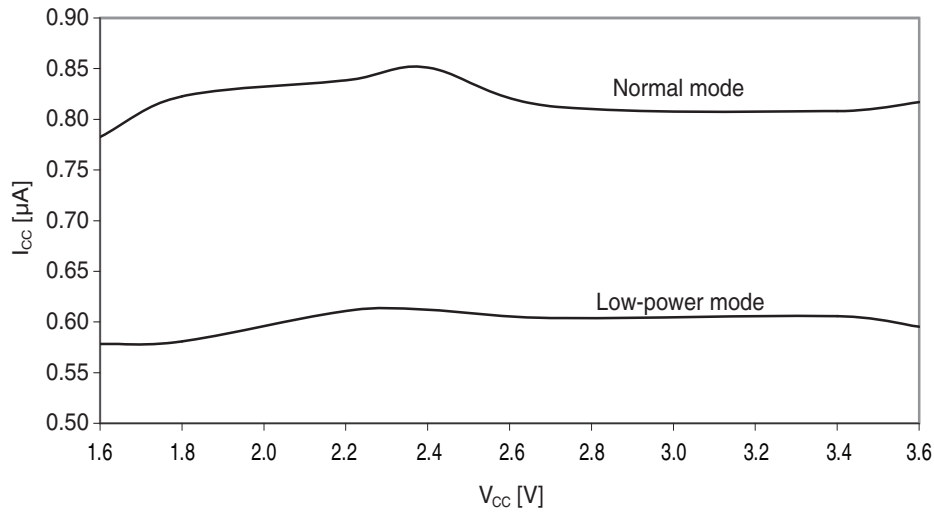
Figure 37-100. Power-save mode supply current vs. V_{CC} .
