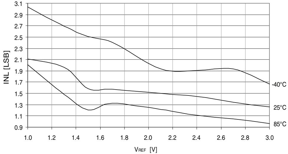
Figure 37-214. DAC INL error vs. V_{REF} .
