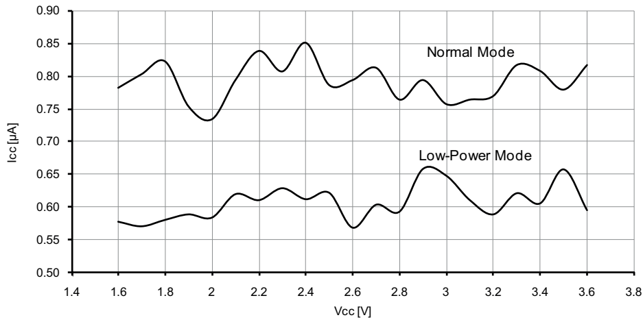
Figure 37-17. Power-save mode supply current vs. V_{CC} . Real Time Counter enabled and running from 1.024kHz output of 32.768kHz TOSC.
