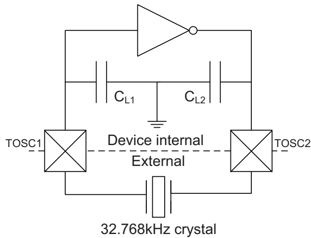
Figure 36-25.TOSC input capacitance.
