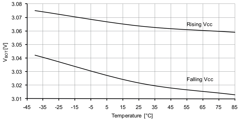
Figure 37-60. BOD thresholds vs. temperature.
