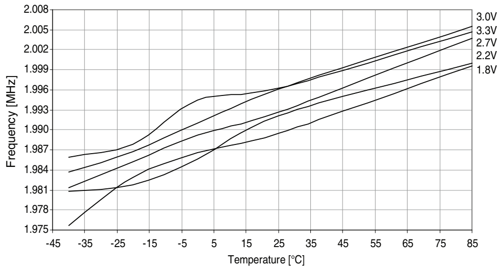
Figure 37-238. 2MHz internal oscillator frequency vs. temperature.
