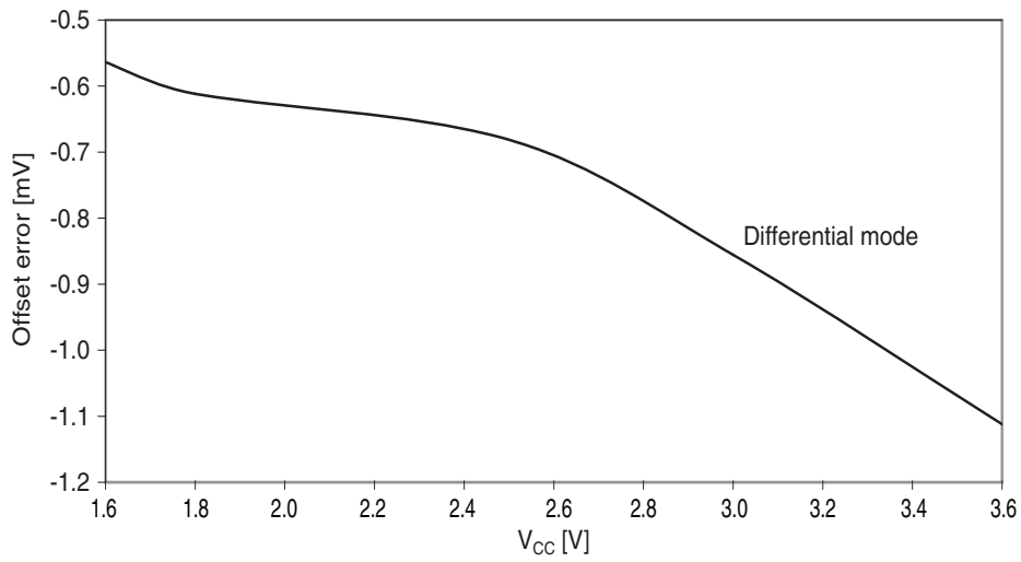
Figure 37-294. Offset error vs. V_{CC} .
