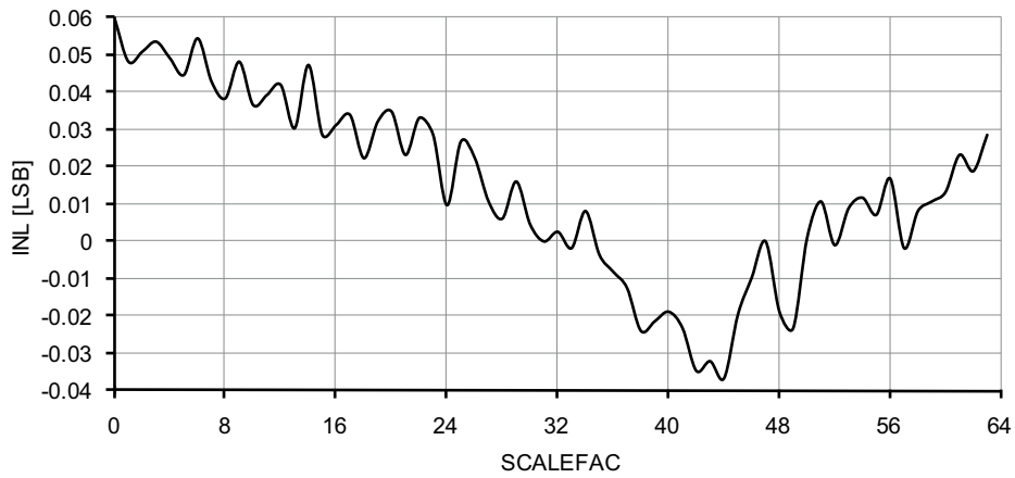
Figure 37-57. Voltage scaler INL vs. SCALEFAC.
