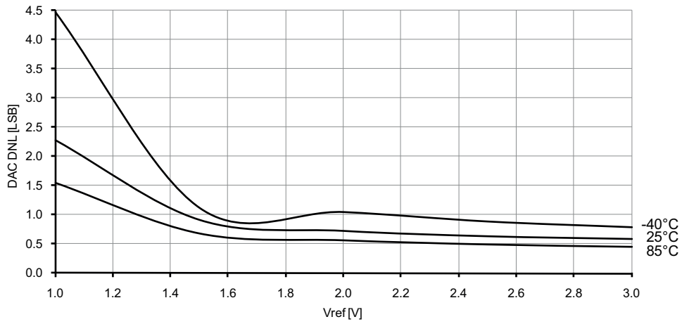
Figure 37-132. DNL error vs. V_{REF} .
