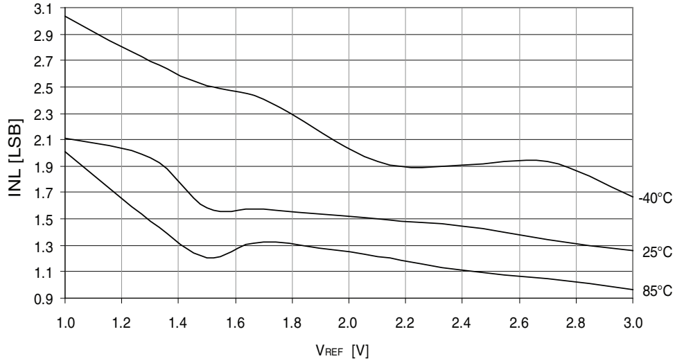
Figure 37-297. DAC INL error vs. V_{REF} .
