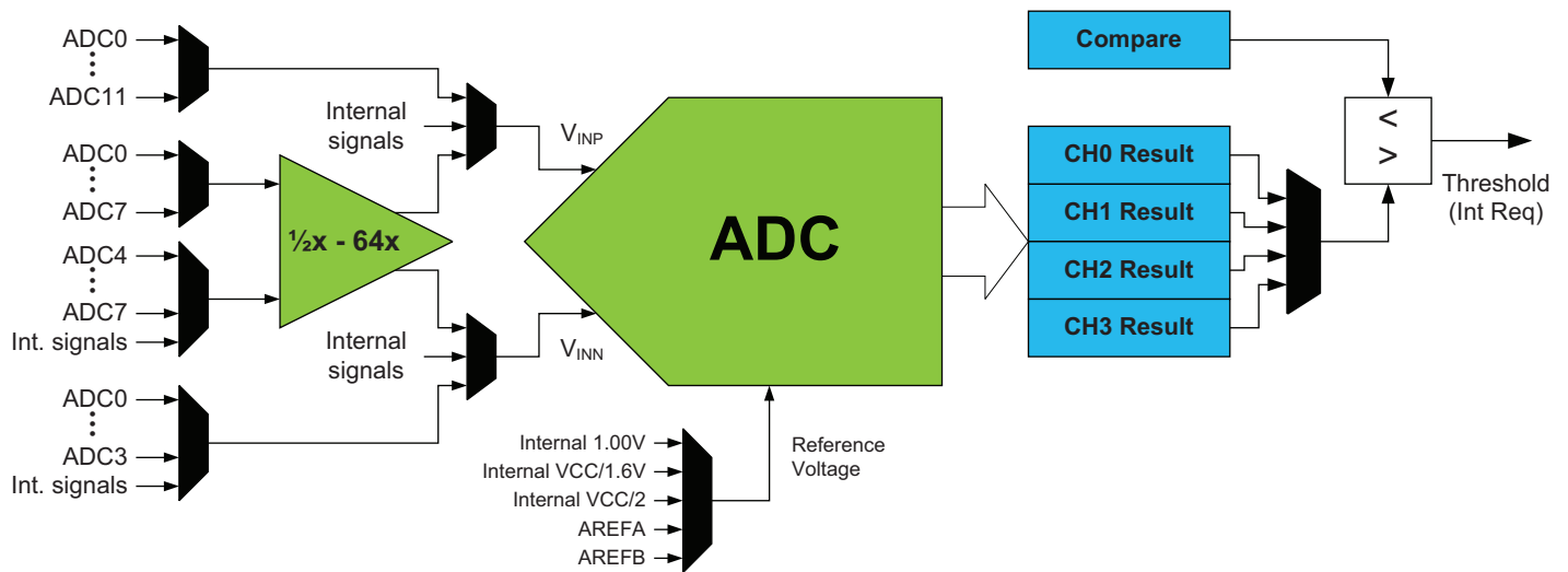
Figure 28-1. ADC overview.
