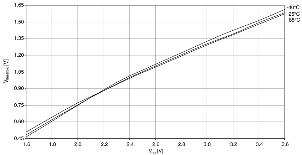
Figure 37-315. Reset pin input threshold voltage vs. V_{CC} .
