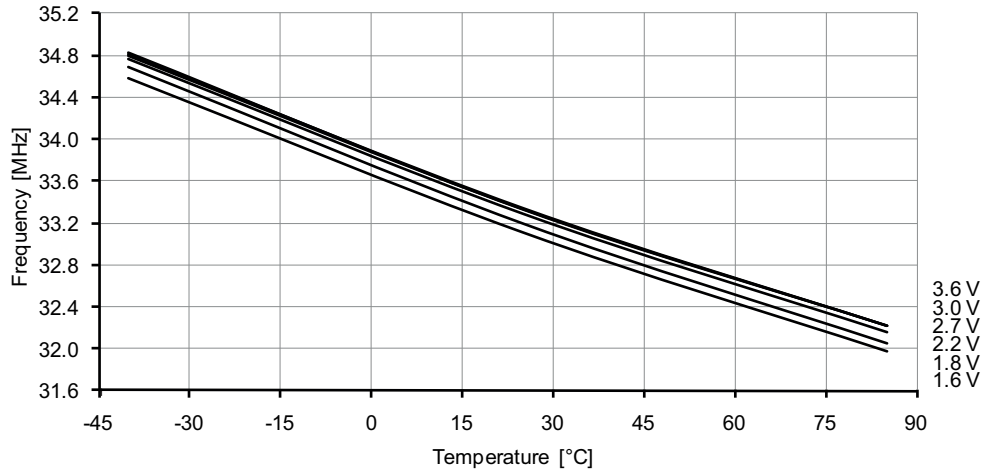
Figure 37-157. 32MHz internal oscillator frequency vs. temperature. DPLL disabled.
