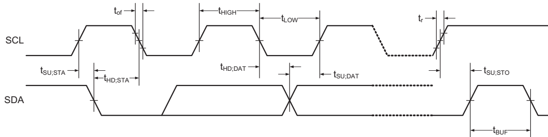
Figure 36-7. Two-wire interface bus timing.
