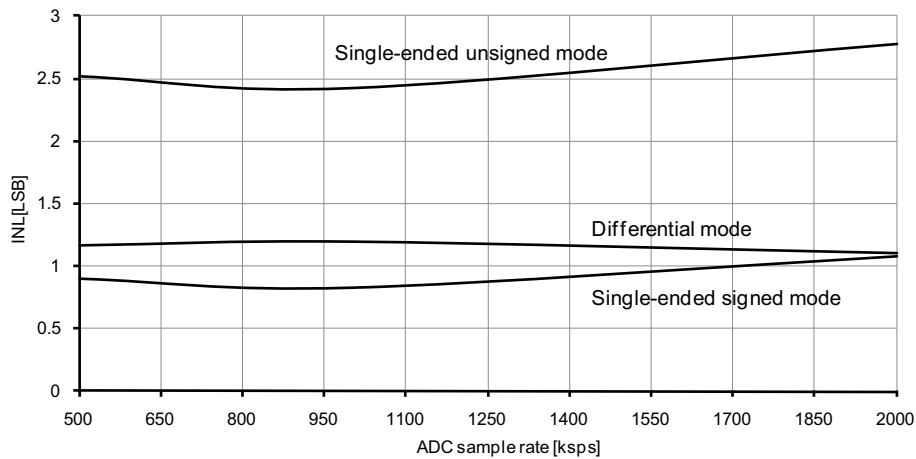
Figure 37-119. INL error vs. sample rate.
