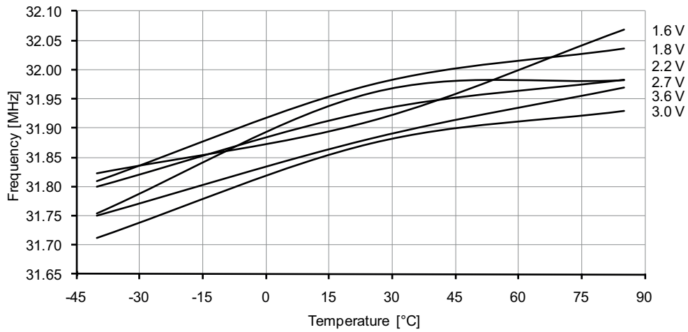
Figure 37-158. 32MHz internal oscillator frequency vs. temperature. DPLL enabled, from the 32.768kHz internal oscillator.
