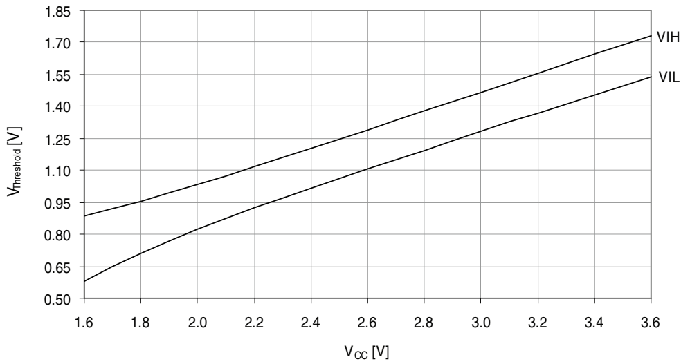
Figure 37-197. I/O pin input threshold voltage vs. V_{CC} . T = 25^{\circ}\text{C} .
