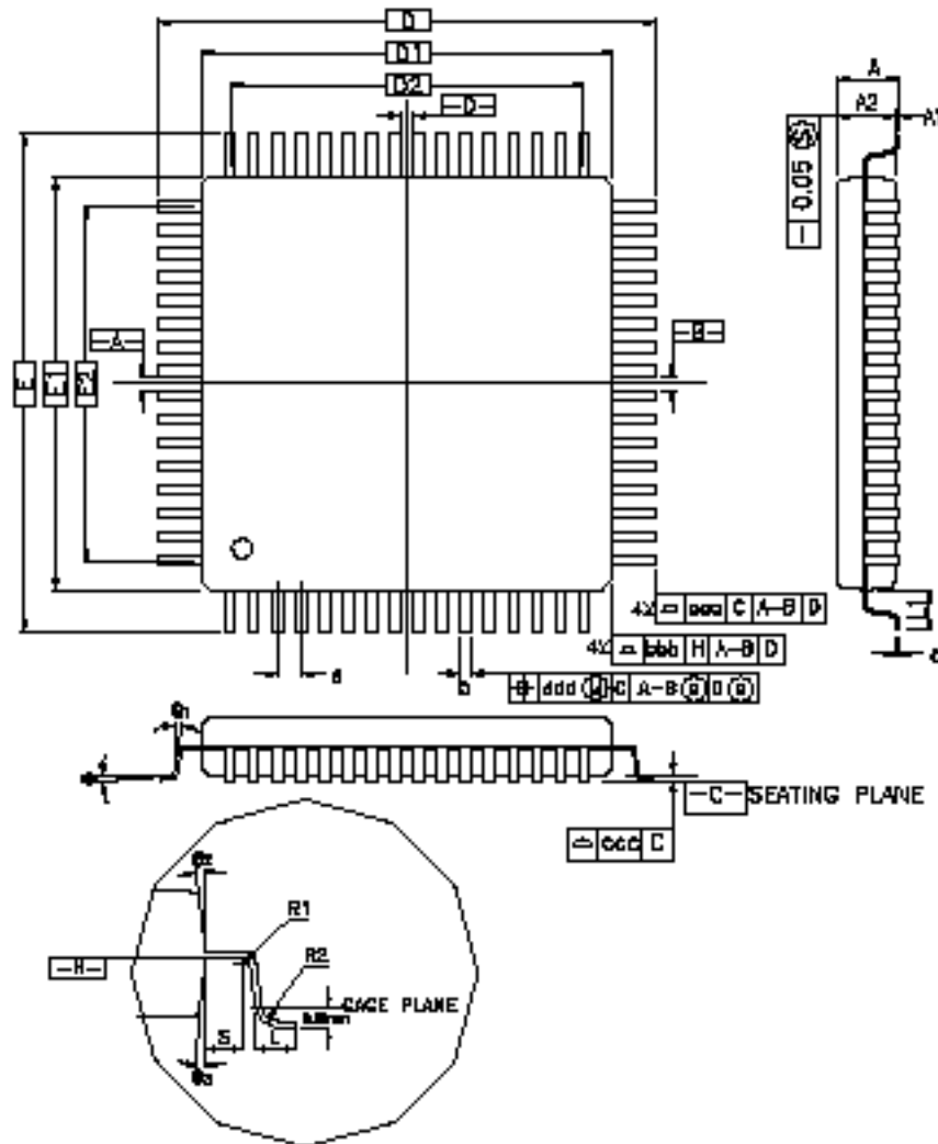
Figure 11-1. 100-lead LQFP Package Drawing
