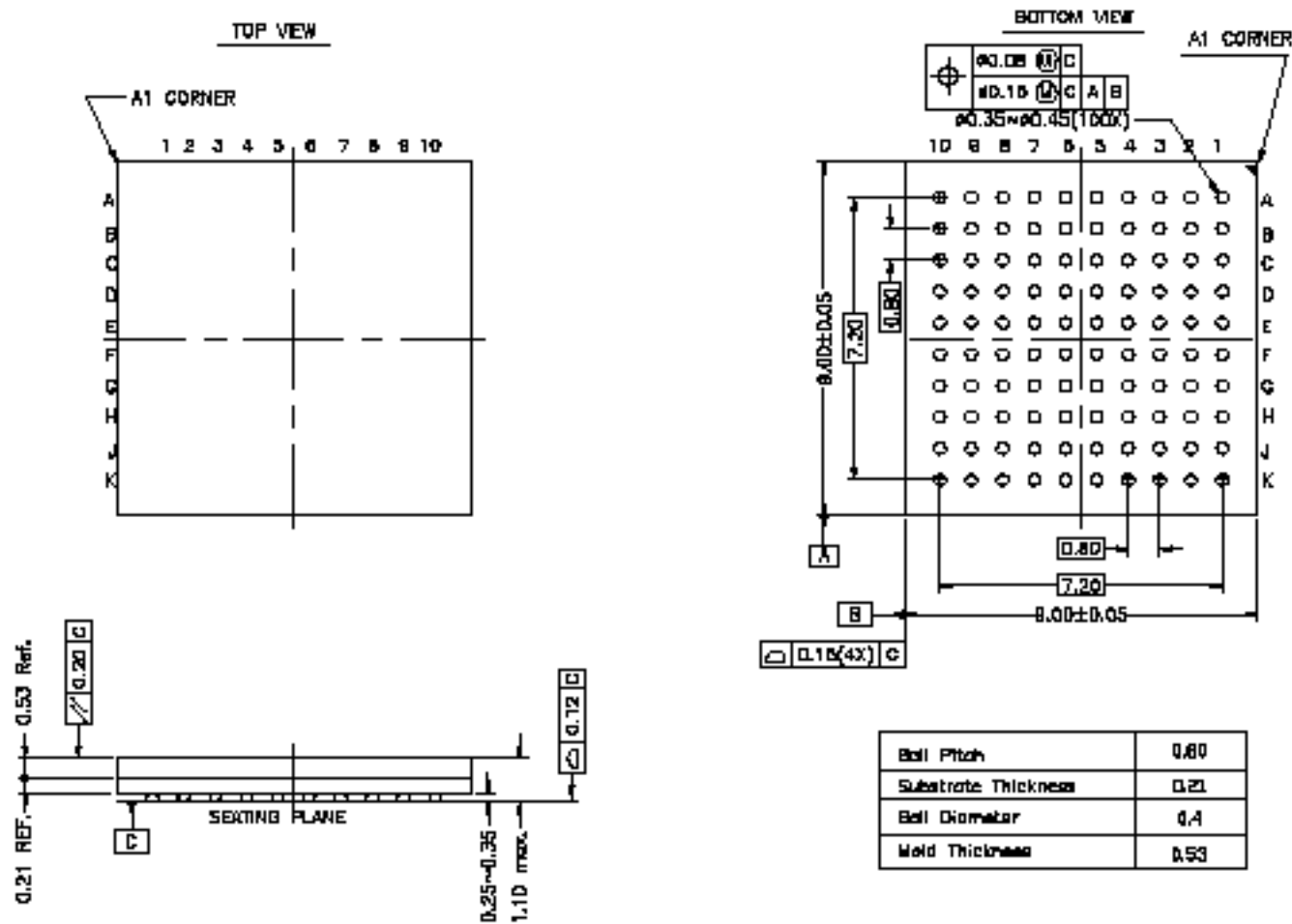
Figure 11-2. 100-ball TFBGA Package Drawing and Dimensions
