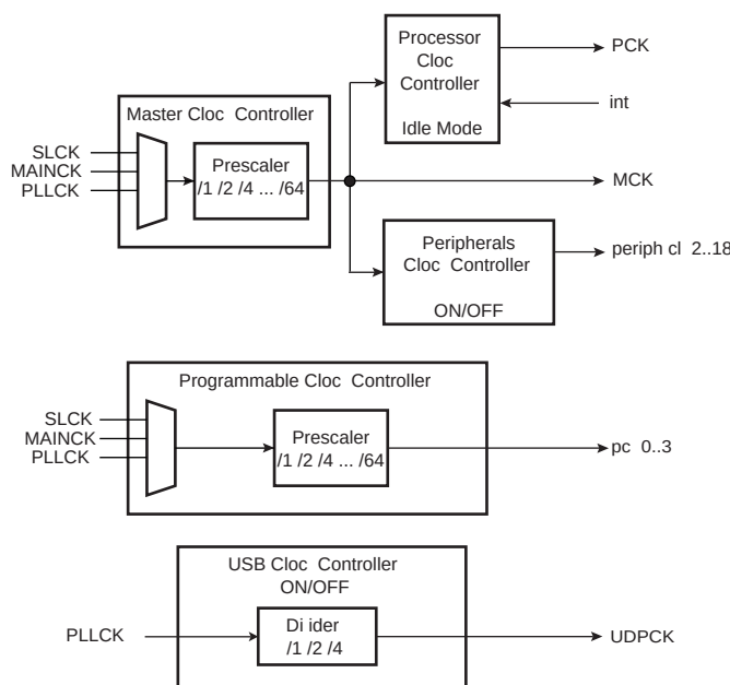
Figure 9-3. Power Management Controller Block Diagram
