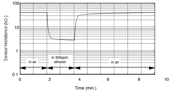
Fig. 10 - Gas response to ethanol
