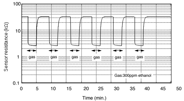
Fig. 11 - Repeatability
