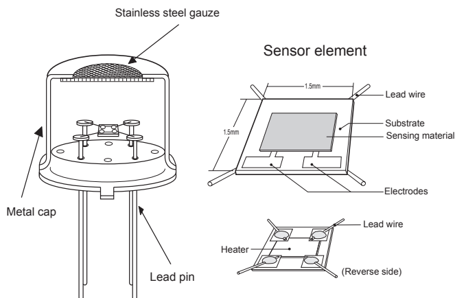
Fig. 1 - Sensor structure
