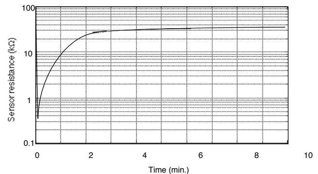
Fig. 12 - Initial action
