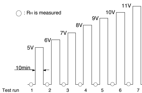
Fig. 19 - Test procedure for heater durability
