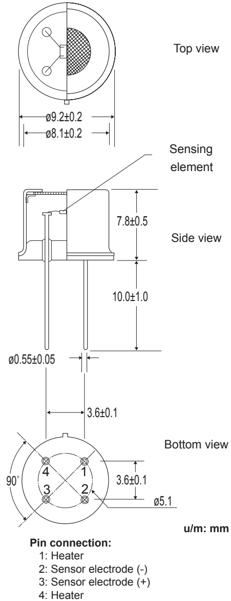
Fig. 3 - Sensor dimensions
