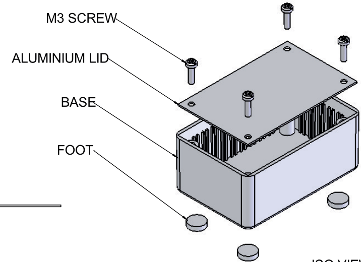
ISO VIEW 1:2
