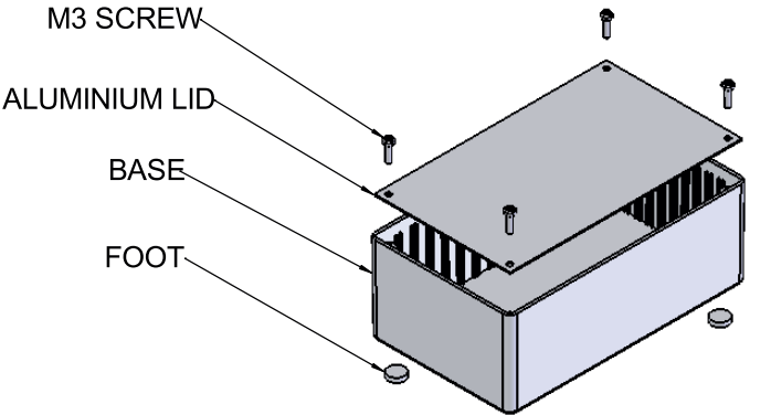
ISO VIEW 1:4
