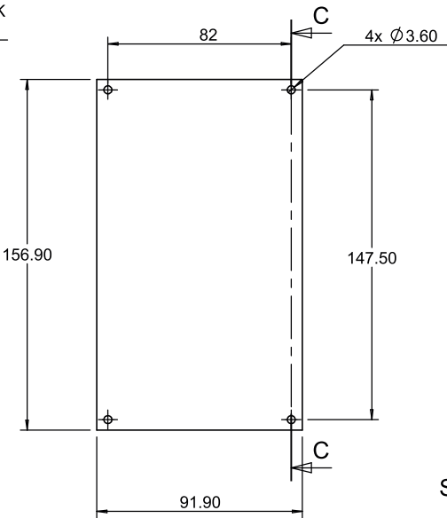
SECTION C-C
