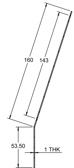
SECTION B-B
