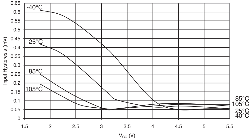
Figure 32-30. ATmega48PA: Reset Pin Input Hysteresis vs. V_{CC}
