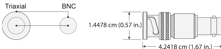
Figure 3: 7078-TRX-GND (CS-712) adapter measurements
