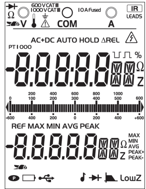
MTX 3291 double 60,000-pts display
