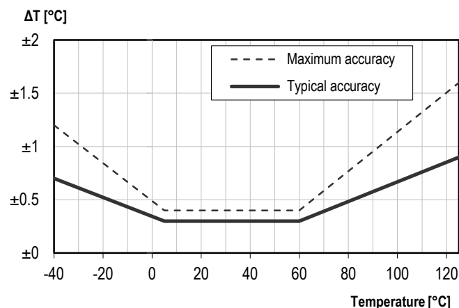
Figure 2 Typical and maximal accuracy for temperature sensor in ^{\circ}\text{C} .
