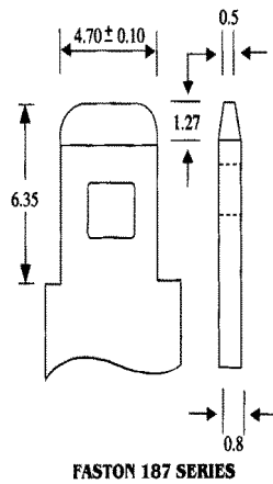
FASTON 187 SERIES
