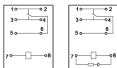
Wiring Diagram
