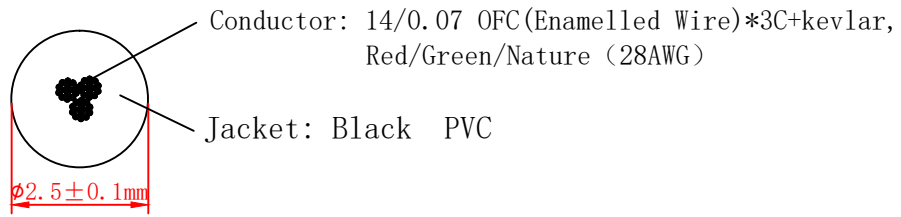
Cable Construction
