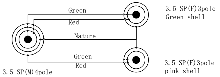
Wiring Method
