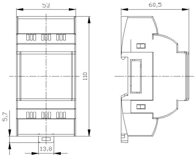
Figure 2. Meter dimensions
