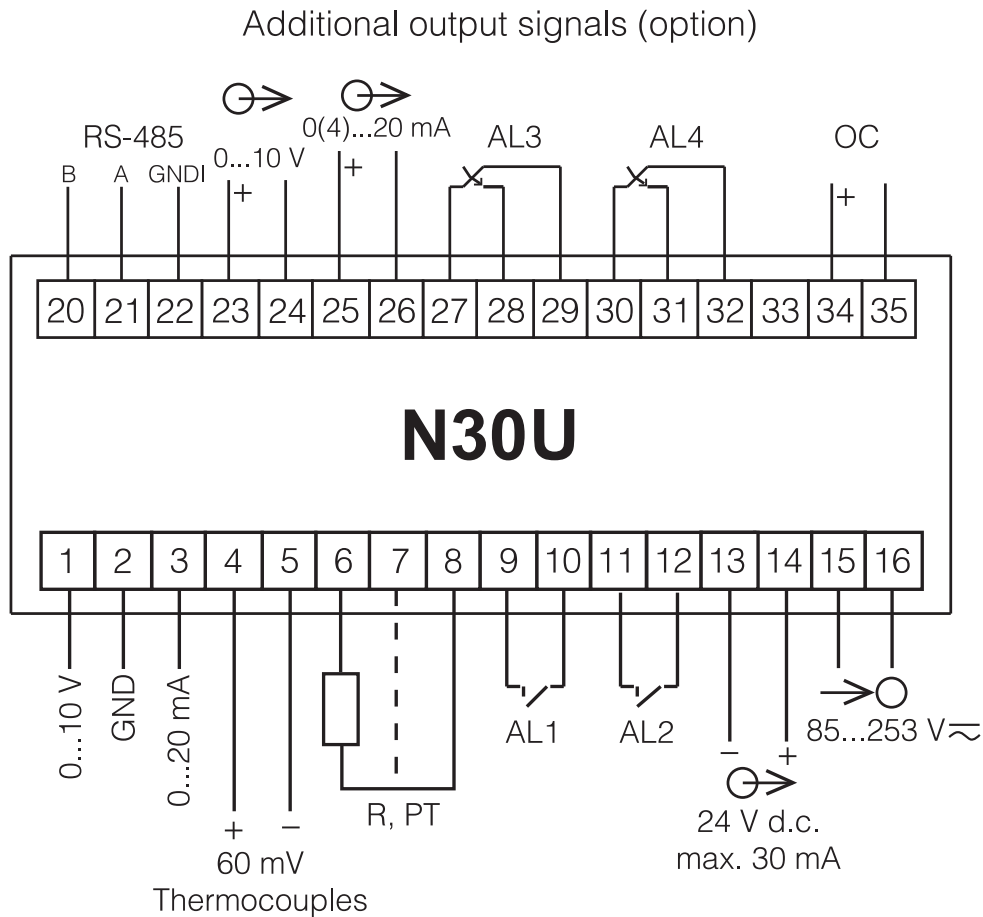
Fig. 4. Description of Signals on Connection Strips
