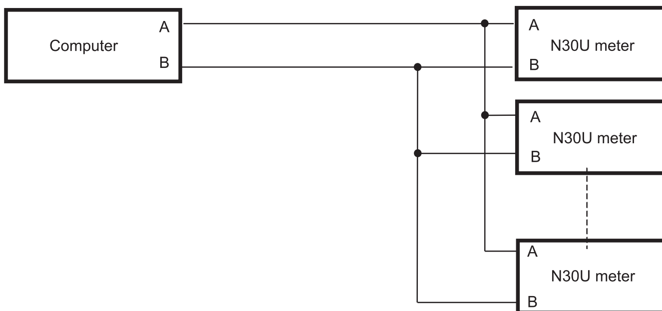
Fig. 12. Connection Way of the RS-485 interface
