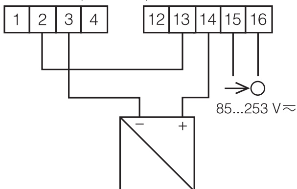
Fig. 5. Ways of the meter Connection
