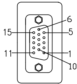
VGA15M
