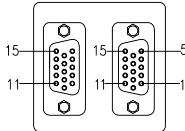
VGA15F VGA15F
