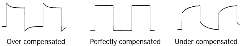
Figure 1-9 Probe Compensation
