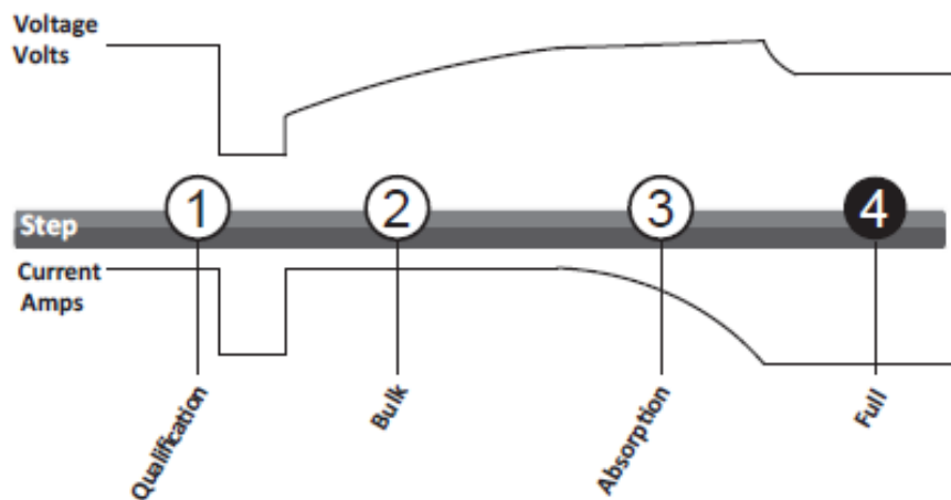
4 Stage LiFePo 4 / LiPO Charge Process
