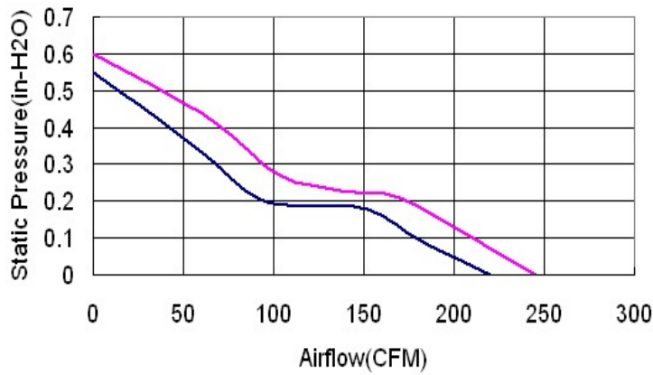
P-Q Curve
