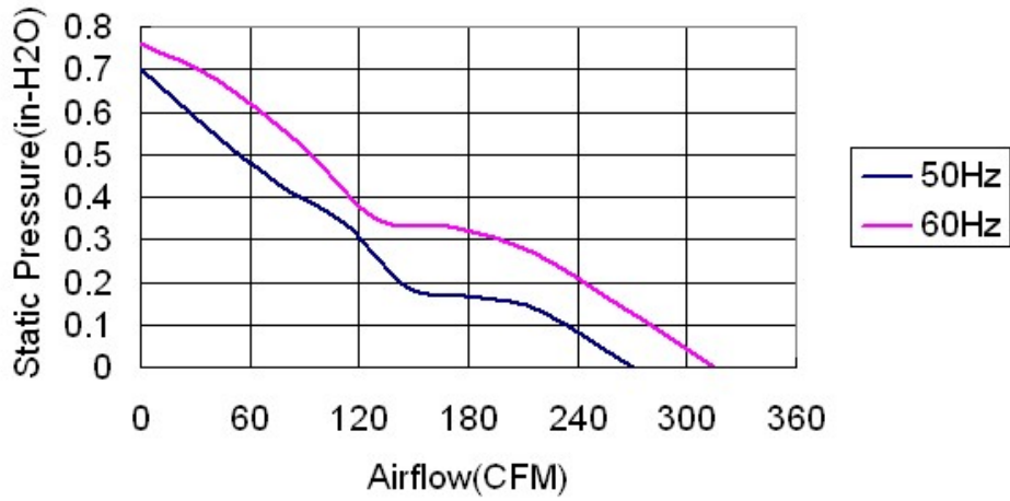
P-Q Curve
