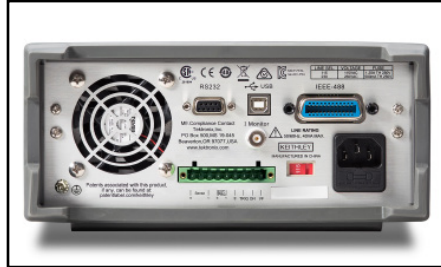
Model 2380-500-15 rear panel
