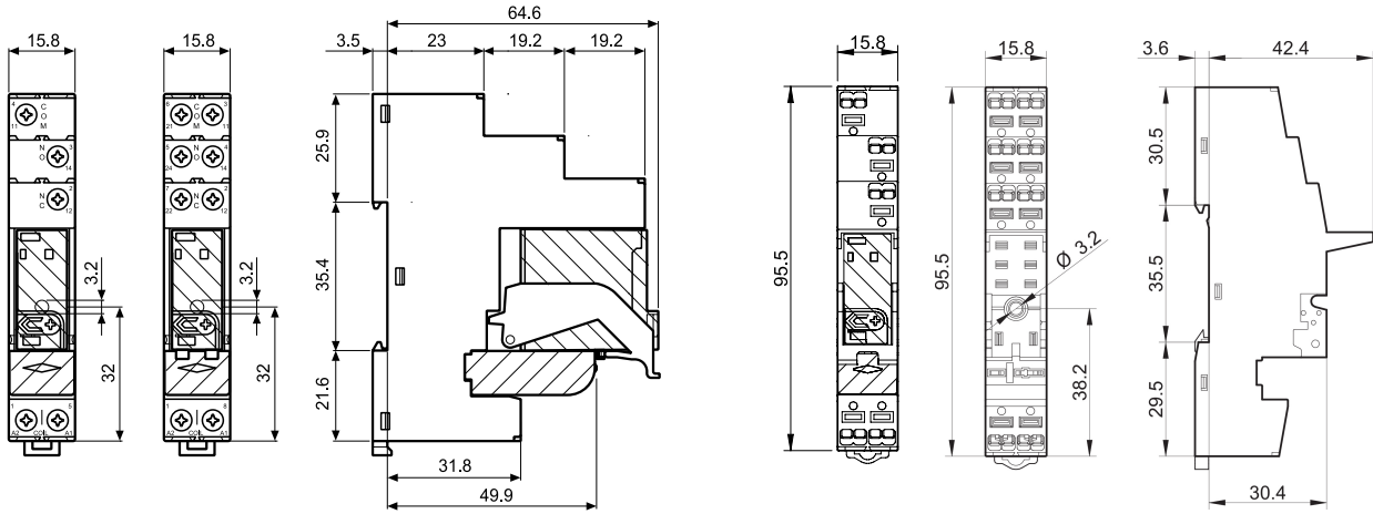
4C.01 / 4C.02 Screw terminals
