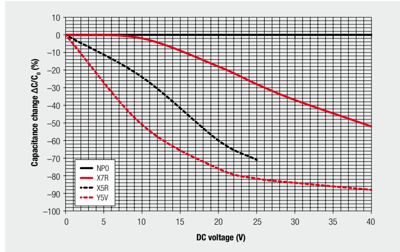
Fig. 2.1: Voltage-dependent capacitance change, example: ceramic capacitors
