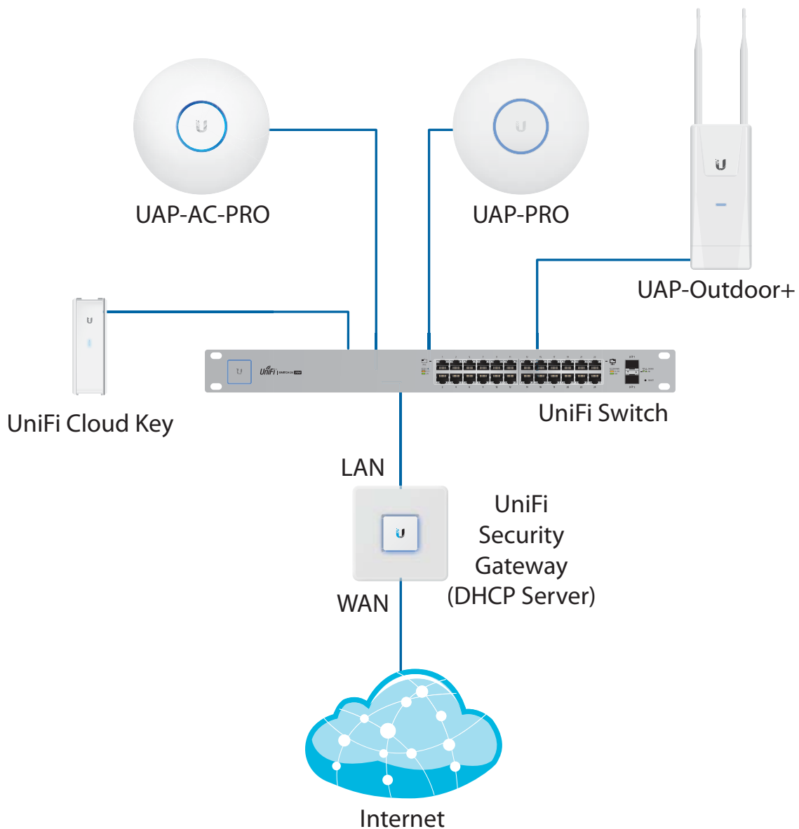
Sample Network Diagram
