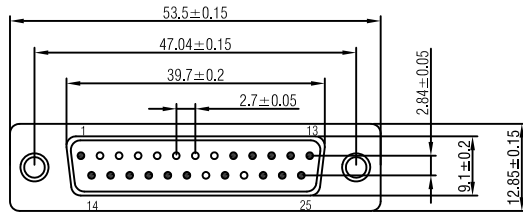
BD25M-DP 9M Mini Adapter(Black Insulator,Nickel Plated)
