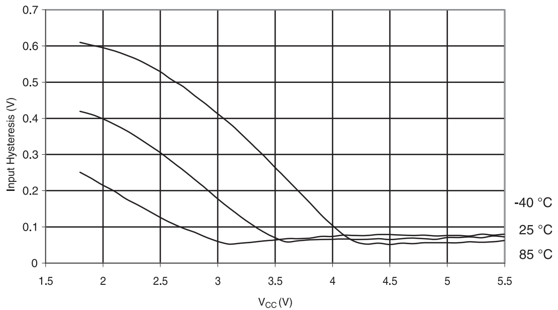
Figure 30-359. ATmega328P: Reset Pin Input Hysteresis vs. V_{CC}
