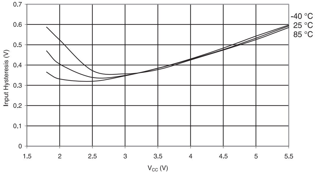
Figure 30-356. ATmega328P: I/O Pin Input Hysteresis vs. V_{CC}
