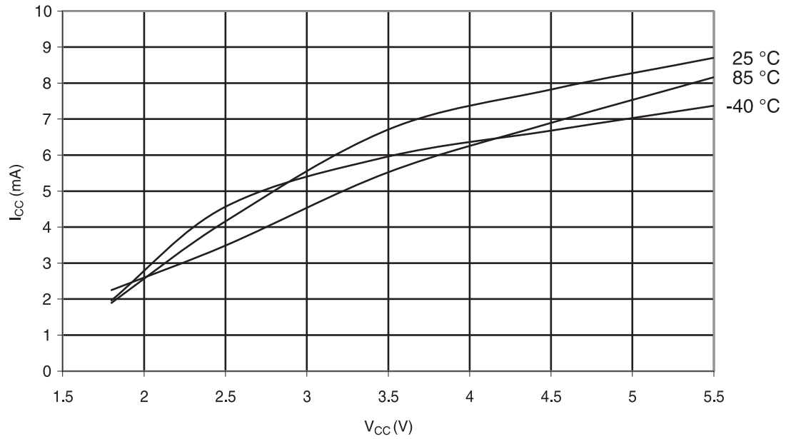
Figure 30-326. ATmega328: Programming Current vs. V_{CC}
