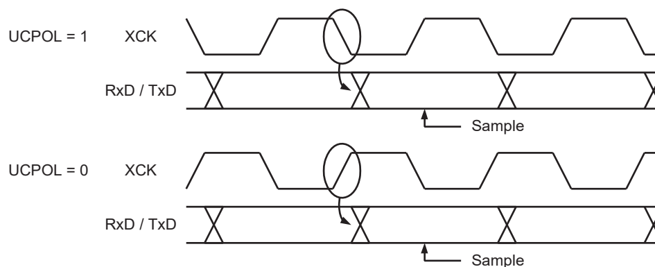
Figure 20-3. Synchronous Mode XCKn Timing.
