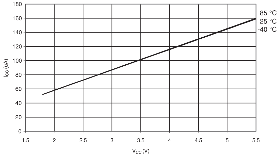
Figure 30-324. ATmega328: AREF External Reference Current vs. V_{CC}
