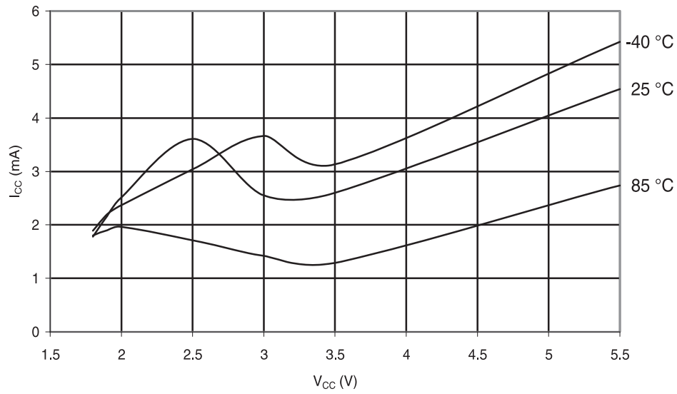
Figure 30-91. ATmega48PA: Programming Current vs. V_{CC}
