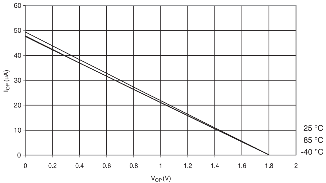
Figure 30-297. ATmega328: I/O Pin Pull-up Resistor Current vs. Input Voltage (V CC = 1.8 V)
