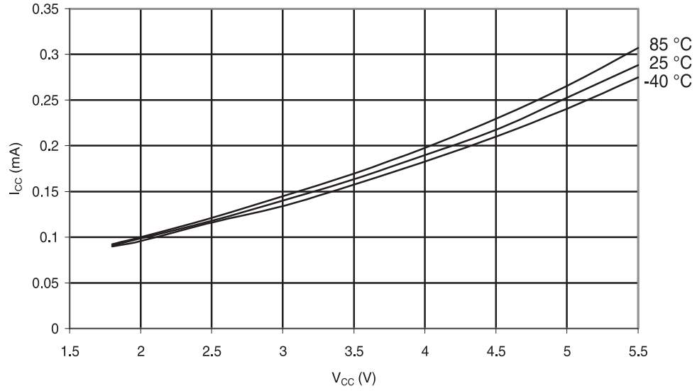
Figure 30-9. ATmega48A: Idle Supply Current vs. V_{CC} (Internal RC Oscillator, 1MHz)
