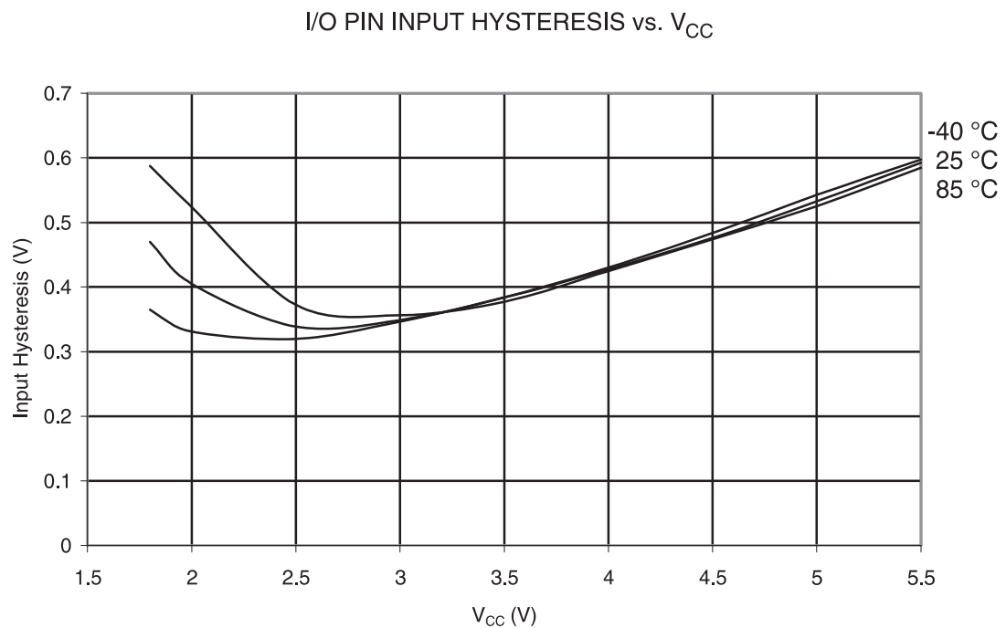
Figure 30-309. ATmega328: I/O Pin Input Hysteresis vs. V_{CC}
