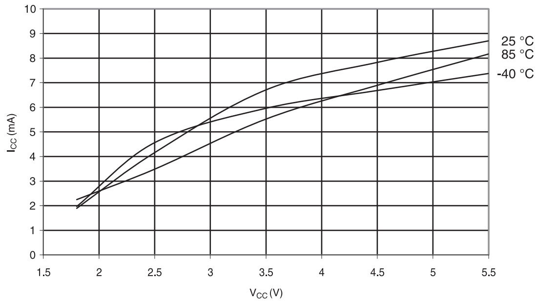
Figure 30-373. ATmega328P: Programming Current vs. V_{CC}
