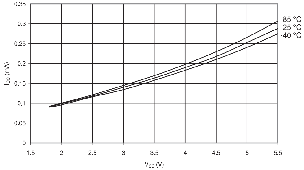
Figure 30-56. ATmega48PA: Idle Supply Current vs. V_{CC} (Internal RC Oscillator, 1MHz)
