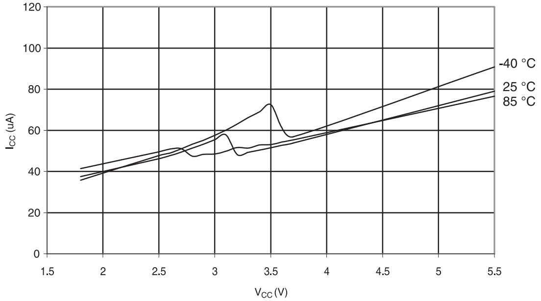
Figure 30-370. ATmega328P: Analog Comparator Current vs. V_{CC}
