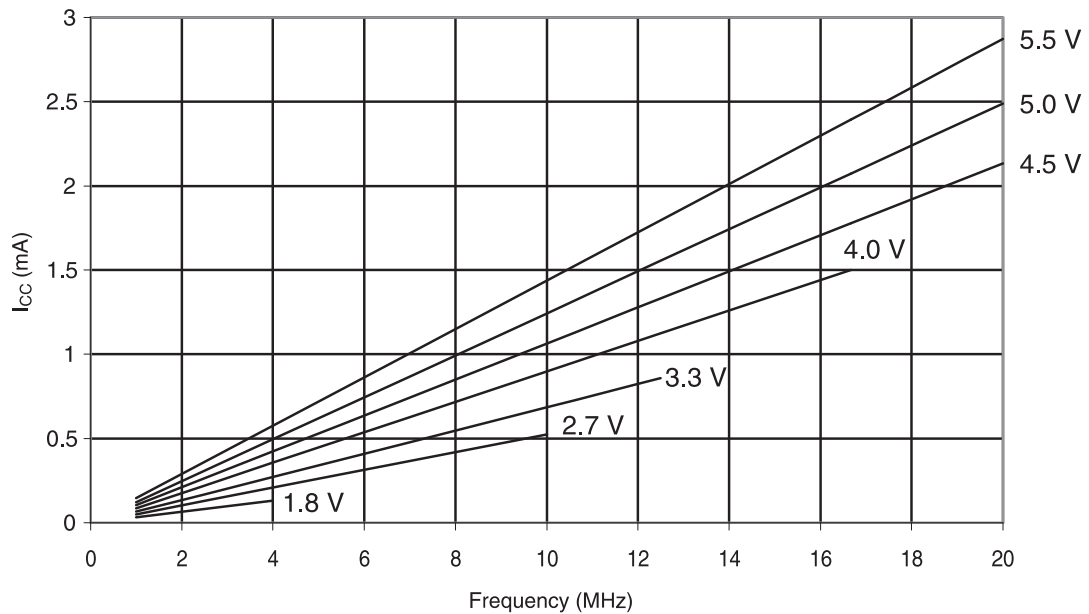
Figure 30-375. ATmega328P: Reset Supply Current vs. Frequency (1 - 20MHz)
