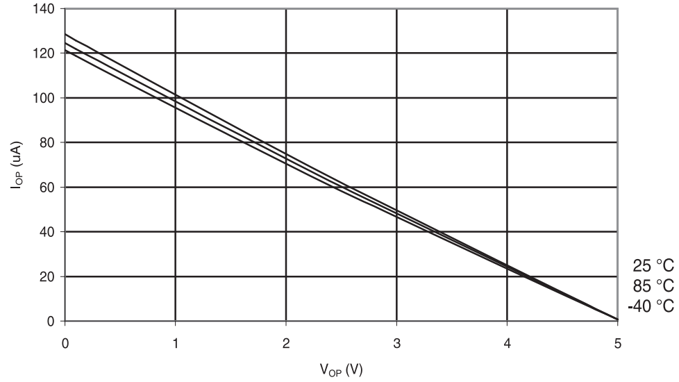
Figure 30-17. ATmega48A: I/O Pin Pull-up Resistor Current vs. Input Voltage ( V_{CC} = 5V )
