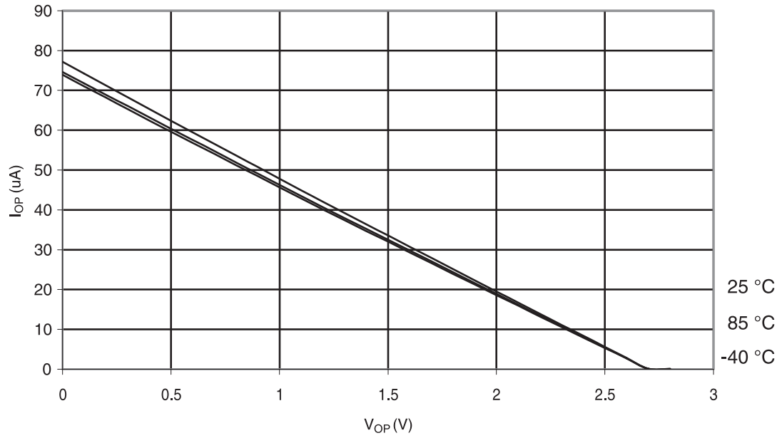
Figure 30-298. ATmega328: I/O Pin Pull-up Resistor Current vs. Input Voltage ( V_{CC} = 2.7\text{ V} )
