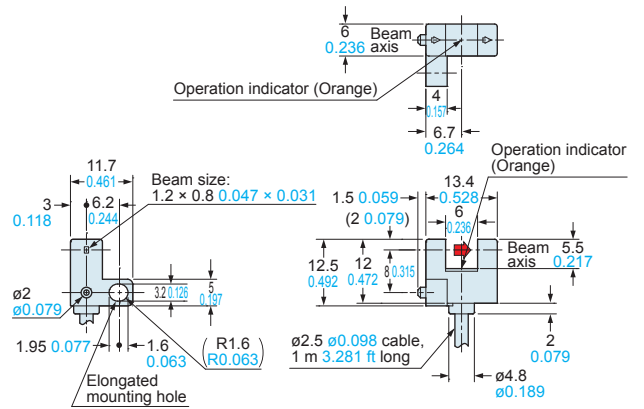
PM-F25 Sensor
