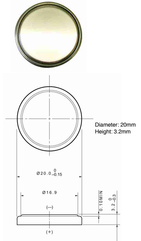
Dimension Drawing
