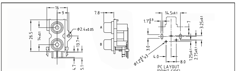
PHS-10B PCB mounting dual RCA Phono connector. Several different coloured inserts available. Nickel Silver or Gold plated finish. PHS-10B (FC684052)
