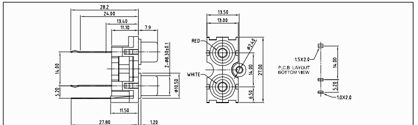
PHS-10A PCB mounting RCA Phono connector. Several different coloured inserts available. Nickel Silver or Gold plated finish. PHS-10A (FC684045)
