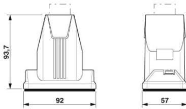
Dimensional drawing
