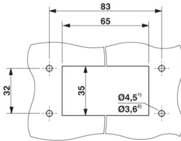
Panel cutout
