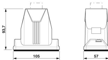
Dimensional drawing
