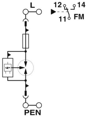
Circuit diagram
