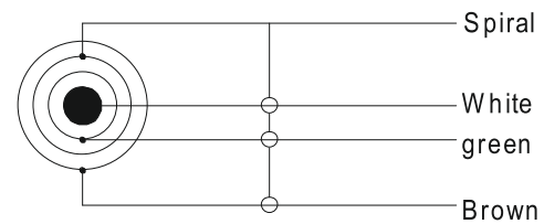
Wiring method
