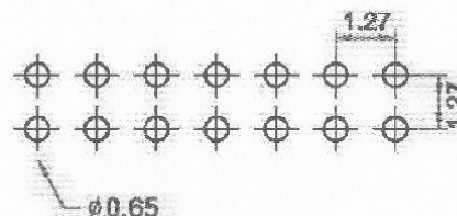
Recommended P.C. Board Hole Layout
