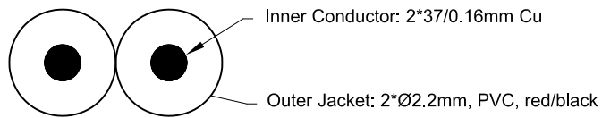
Cable Structure (0.75mm 2 )
