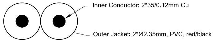
Cable Structure (0.4mm 2 )
