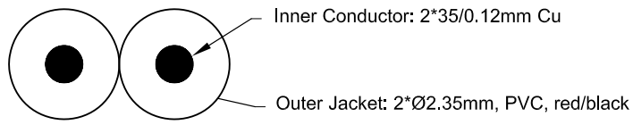
Cable Structure
