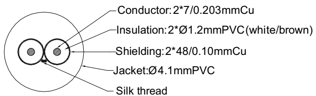
Cable section
