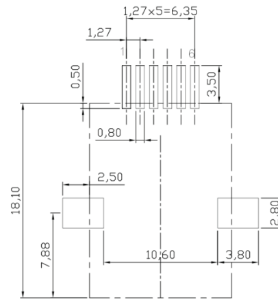
PCB Layout Component Side Shown
